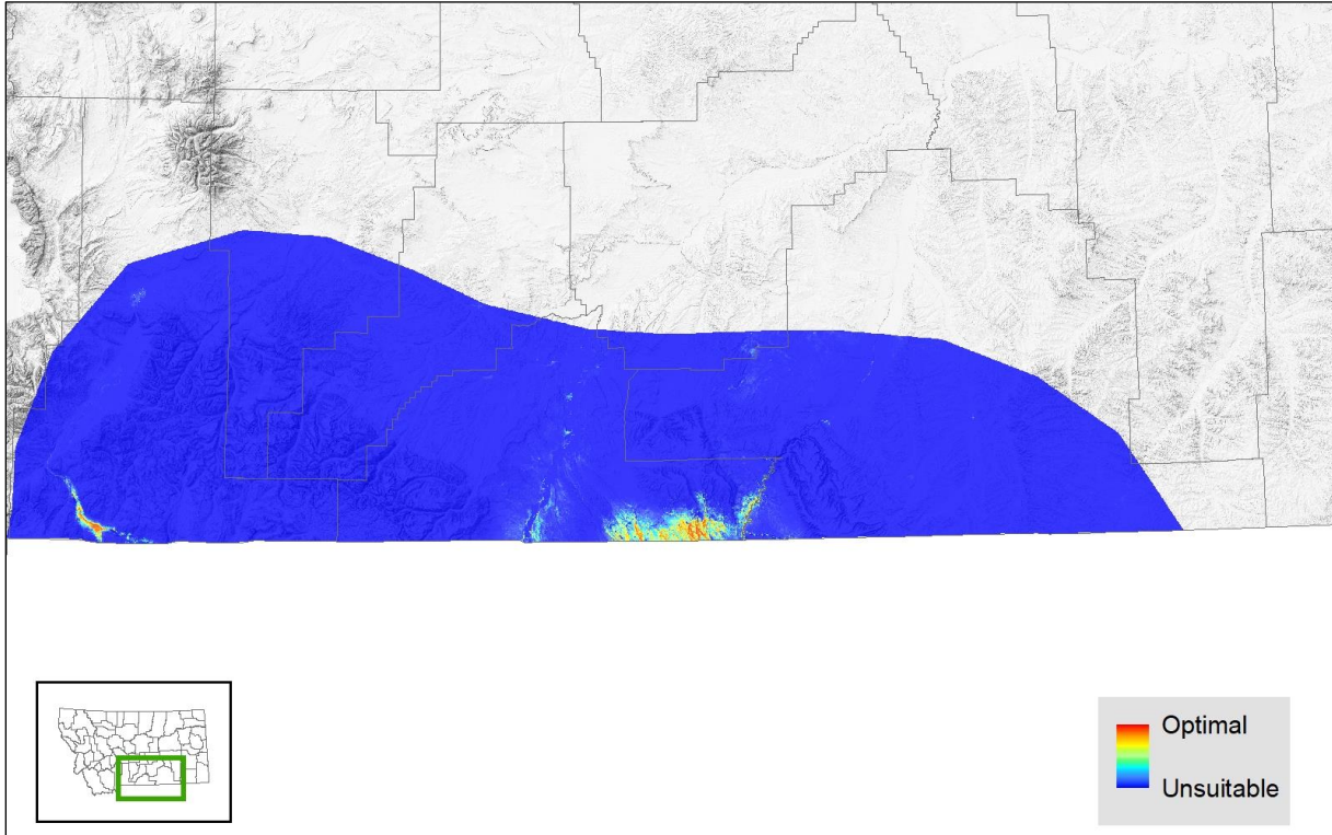
Figure 4. Continuous habitat suitability model logistic output (90-meter pixels); white area is not modeled.
